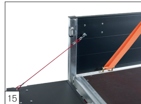
Standard: TÜV certified HAPERT load-securing system. These binding brackets are integrated in the sides with a capacity of 1000 daN each.
